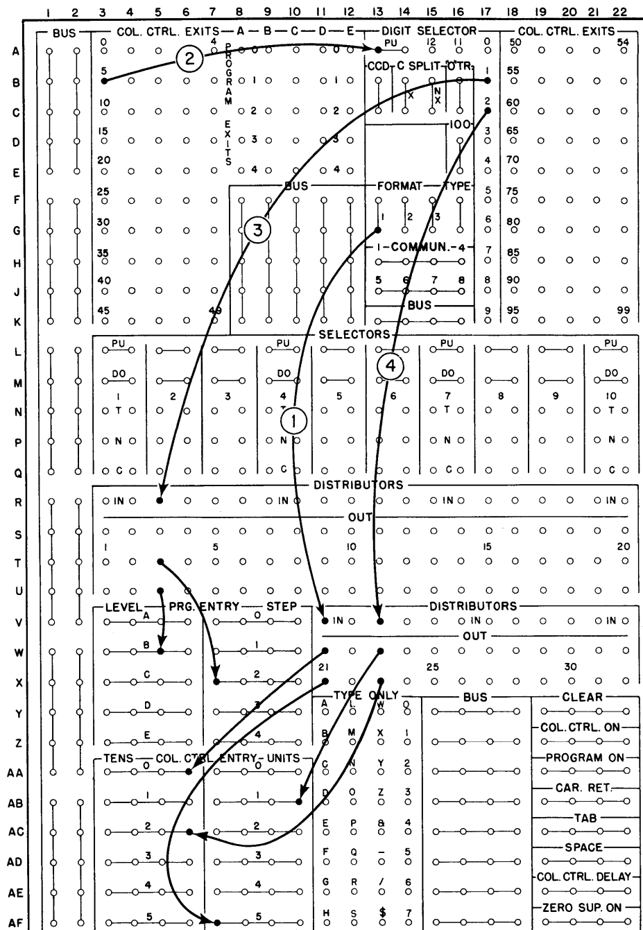
Figure 67. Alteration of Format Control
