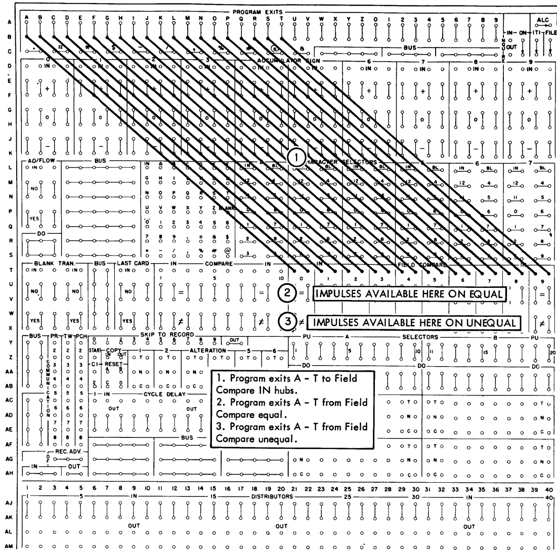
Figure 119. Program Exit Expansion-Field Compare Selectors
