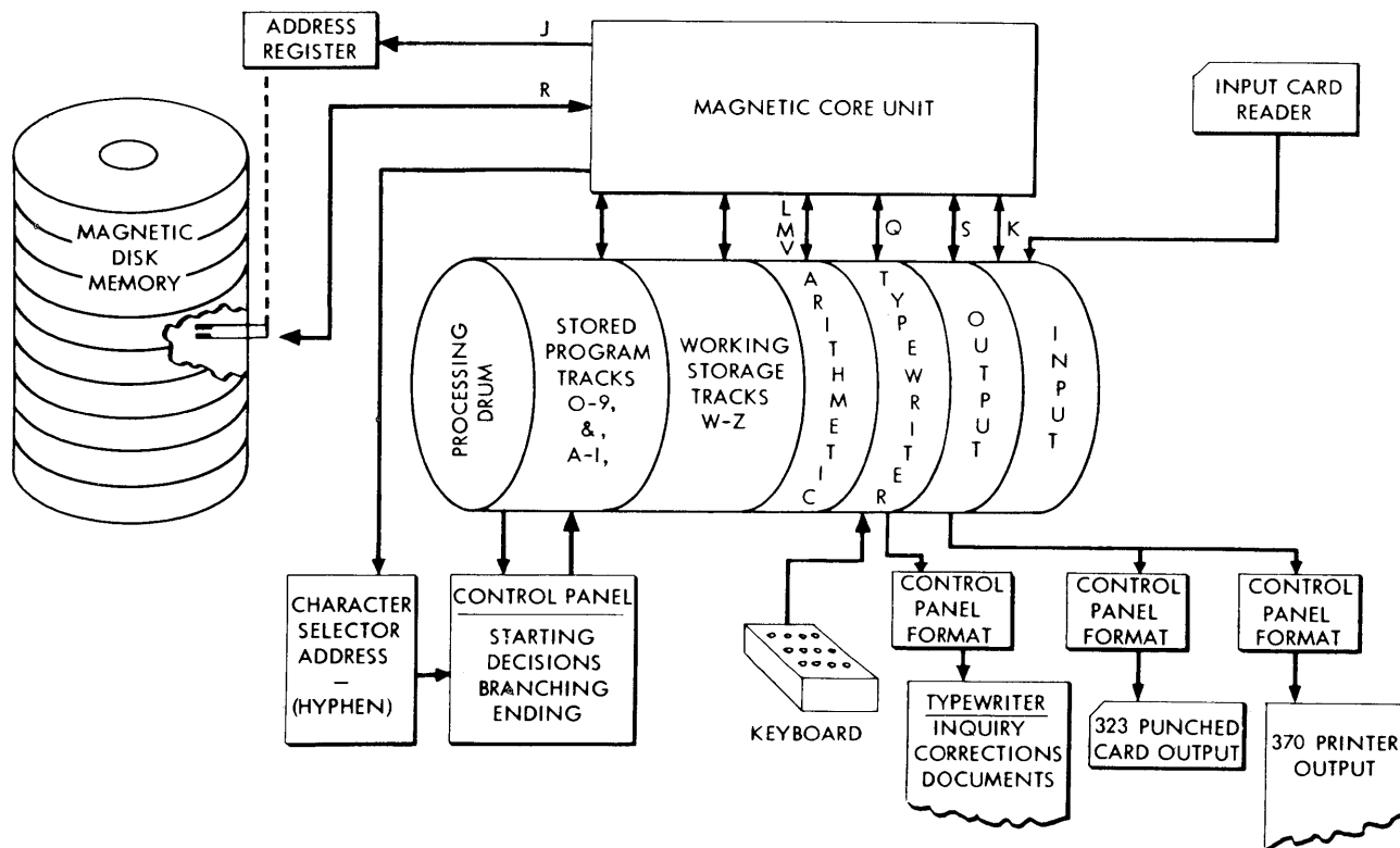
Figure 5. Summary of the 305 System
