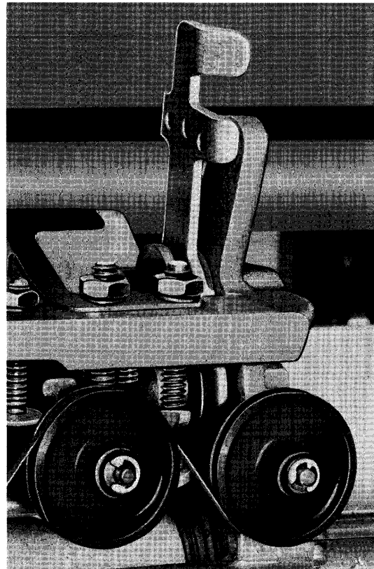
Figure 91. Forms Thickness Adjustment Device
