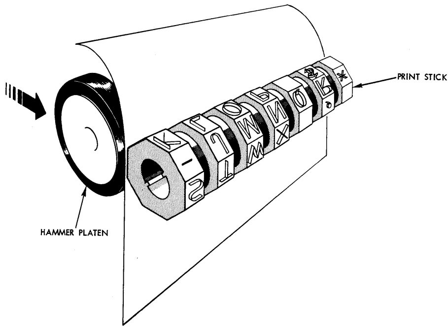
Figure 75. Print Stick and Platen
