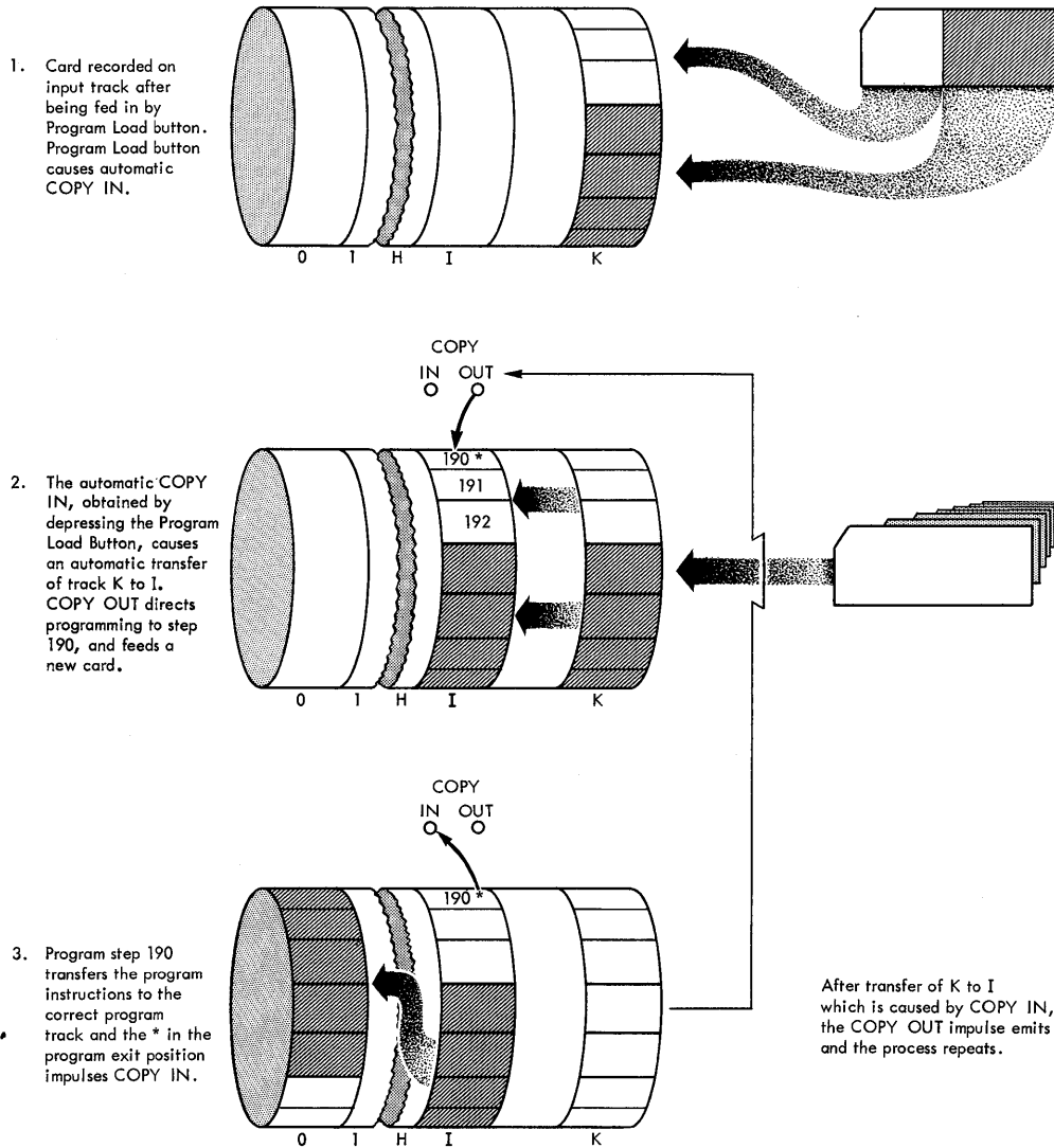
Figure 14. Program Loading
