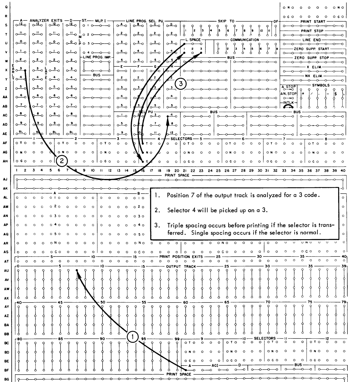
Figure 97. Selective Spacing
