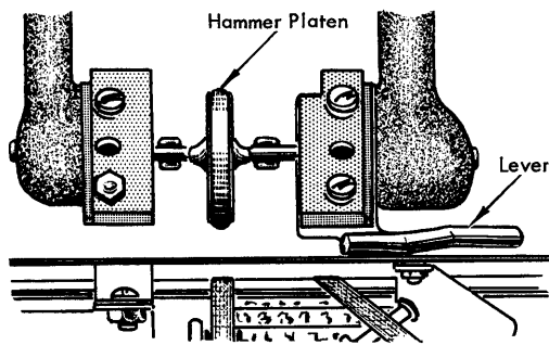
Figure 92. Printer Platen
