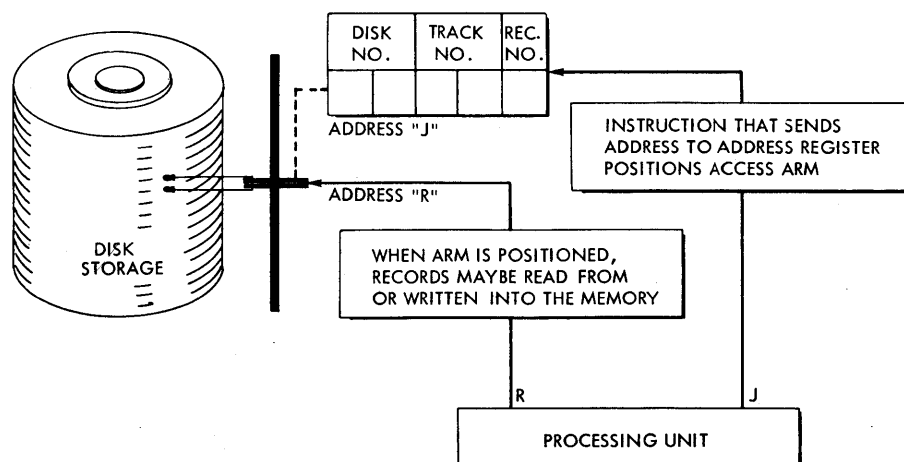
Figure 17. Method of Addressing, Reading and Writing in Disk Storage
