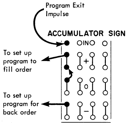
Figure 7. Method of Branching by Control Panel Wiring
