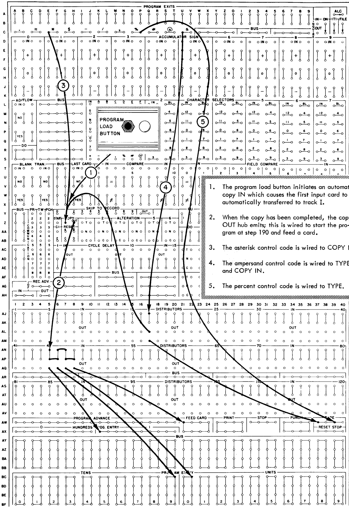
Figure 16. Control Panel Wiring for Loading the Program
