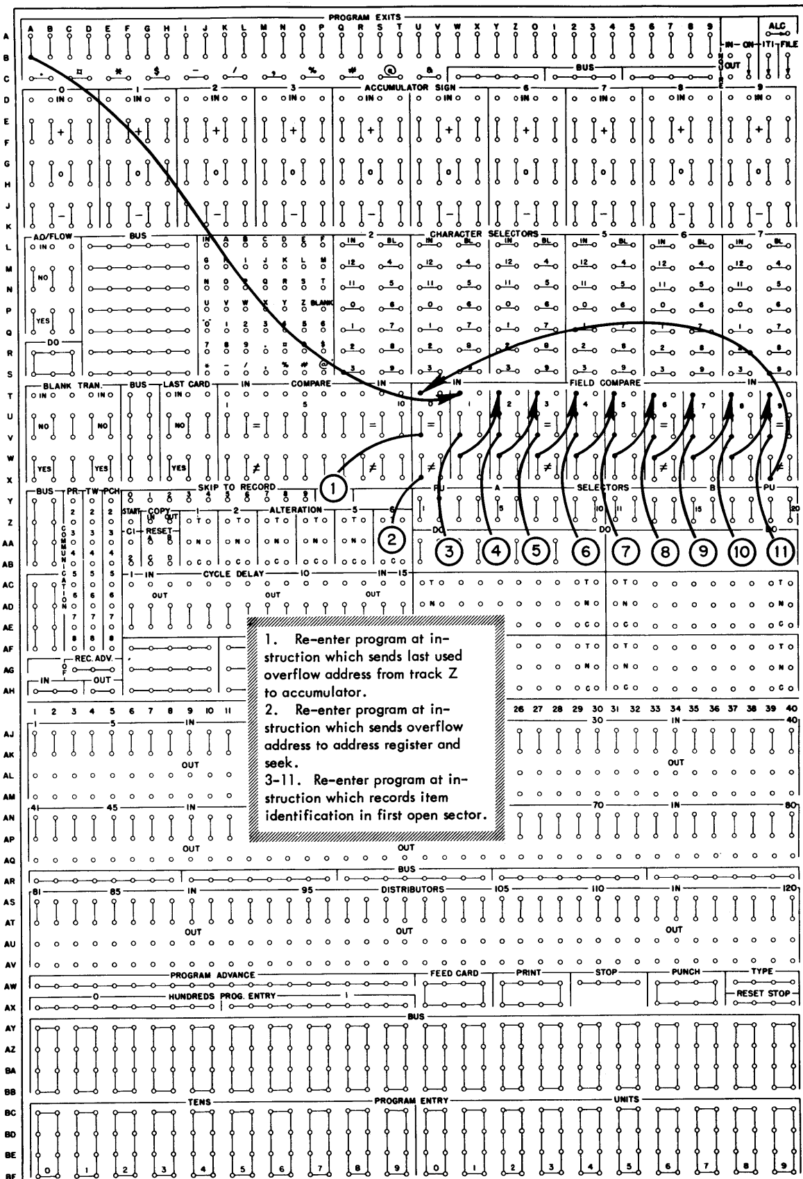
Figure 38. Wiring Diagram-Constructing an Index Record and Storing a Record (Part 1)
