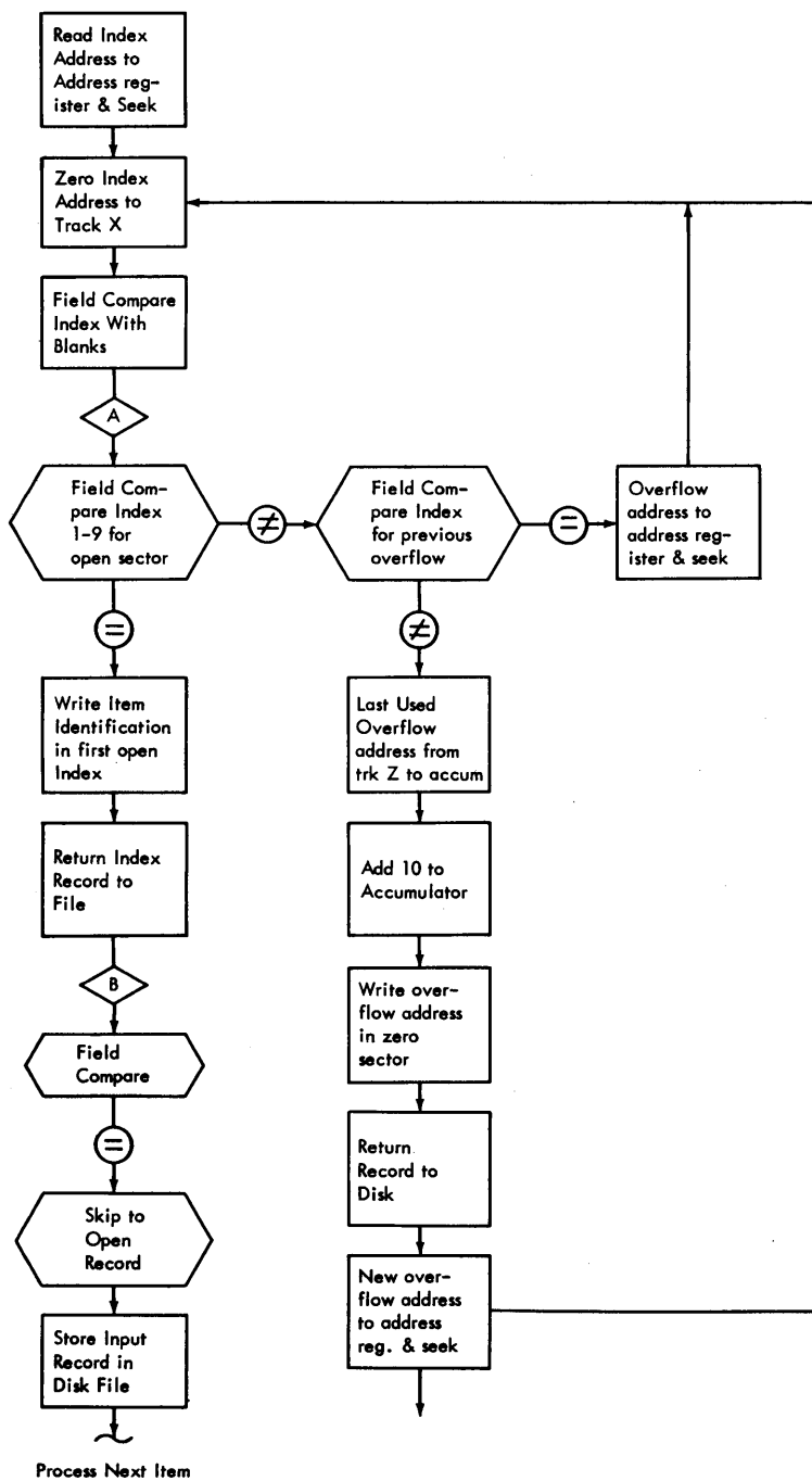
Figure 37. Constructing an Index Record and Storing a Record (Block Diagram)
