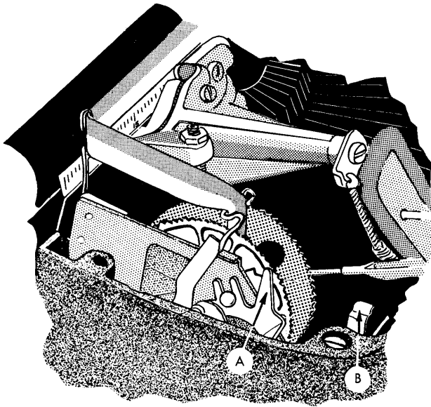
Figure 71. Ribbon Reverse
