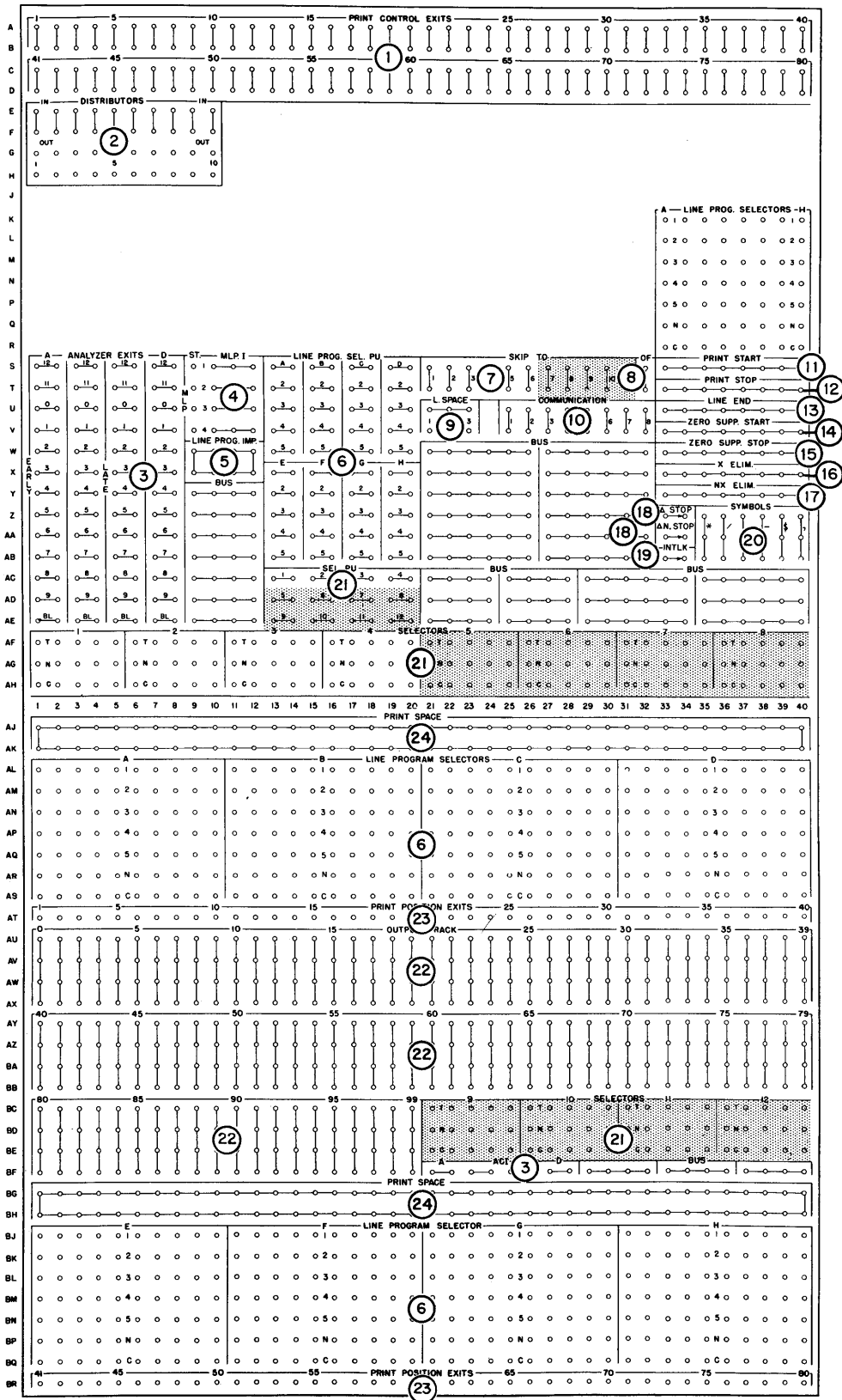
Figure 143. 370 Printer Control Panel
