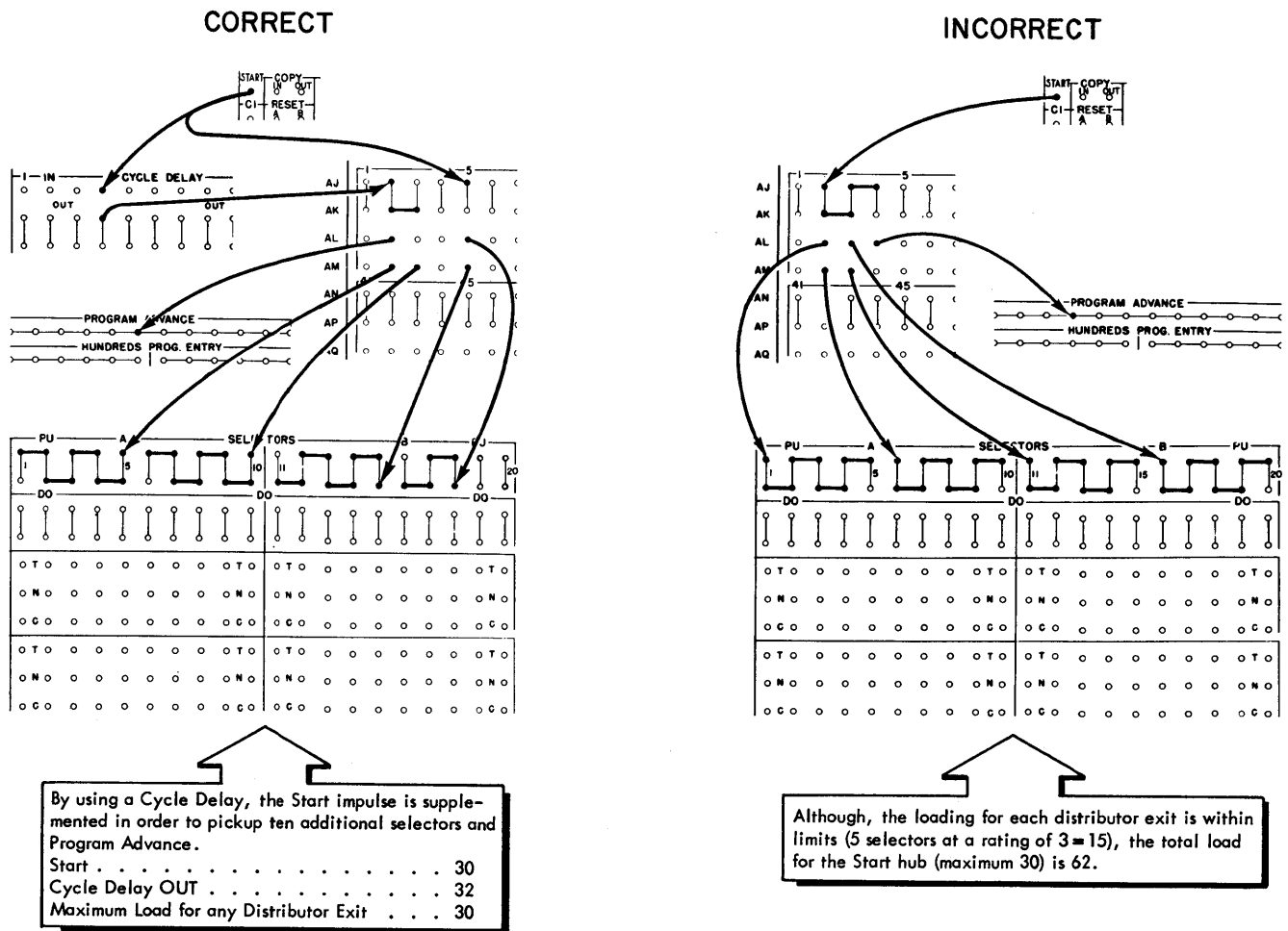
Figure 115. Wiring Based Upon Load Chart Ratings
