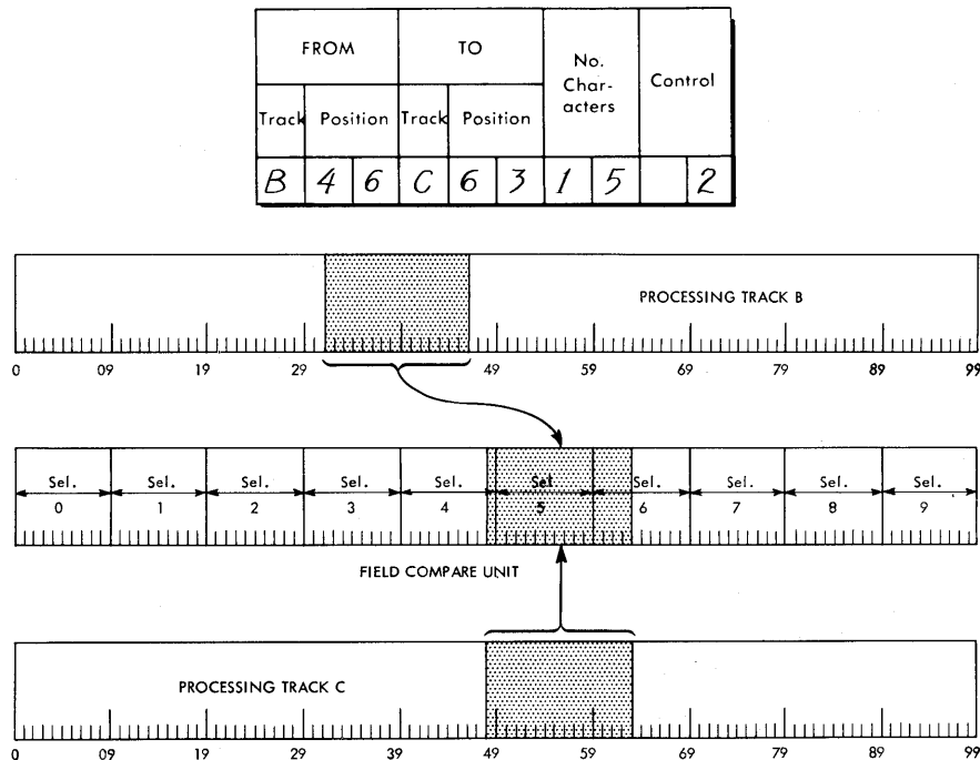
Figure 19. Schematic of a Field Compare Operation
