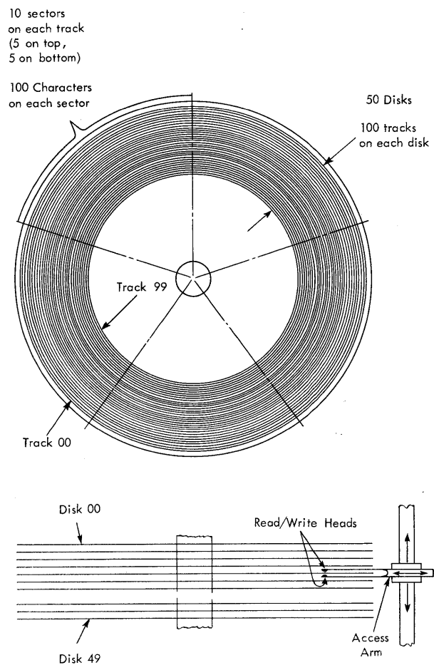
Figure 4. Schematic Disk Storage
