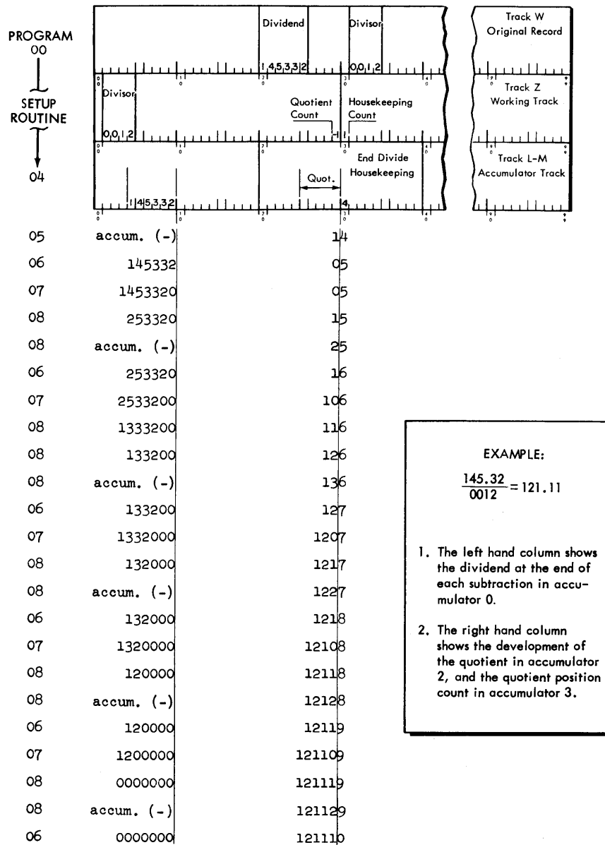
Figure 27. Division by Successive Subtraction (Example)
