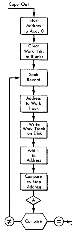
Figure 28. Block Diagram for Clearing Disk Storage
