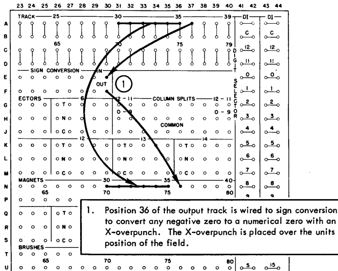
Figure 106. Sign Conversion
