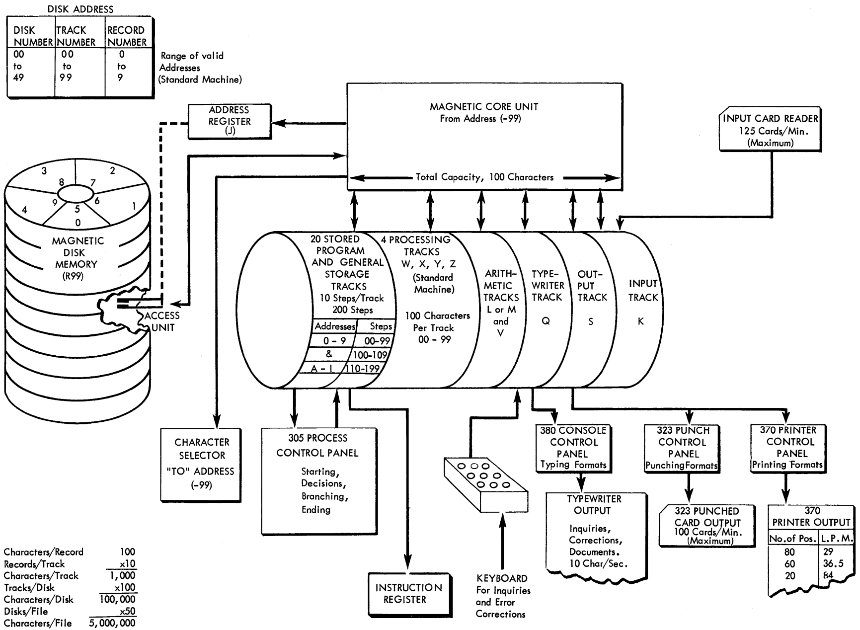
Figure 149. Summary of the 305 System
