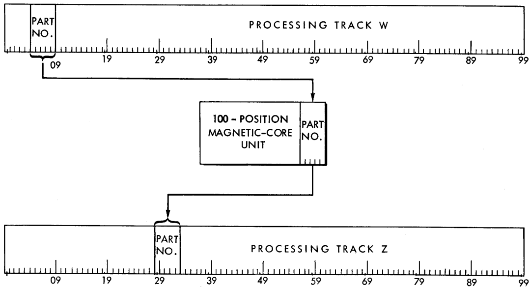
Figure 10. Schematic of a Normal Transfer Operation
