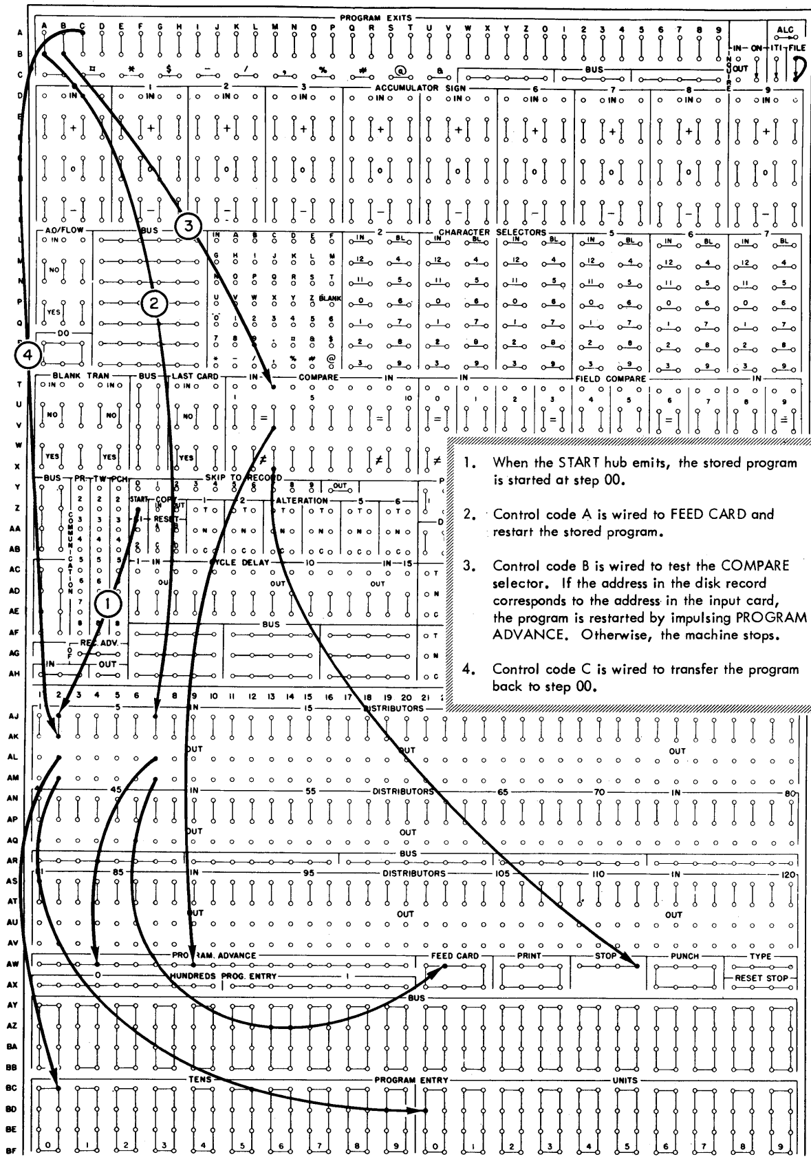
Figure 33. Control Panel Wiring for Loading Disk Storage
