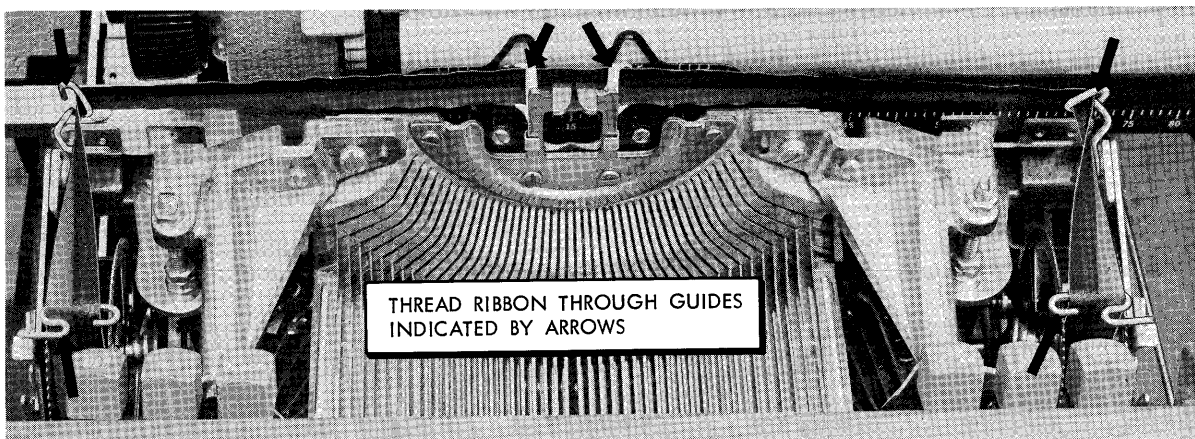
Figure 72. Typewriter Ribbon
