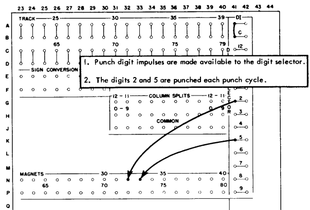
Figure 112. Digit Emitting
