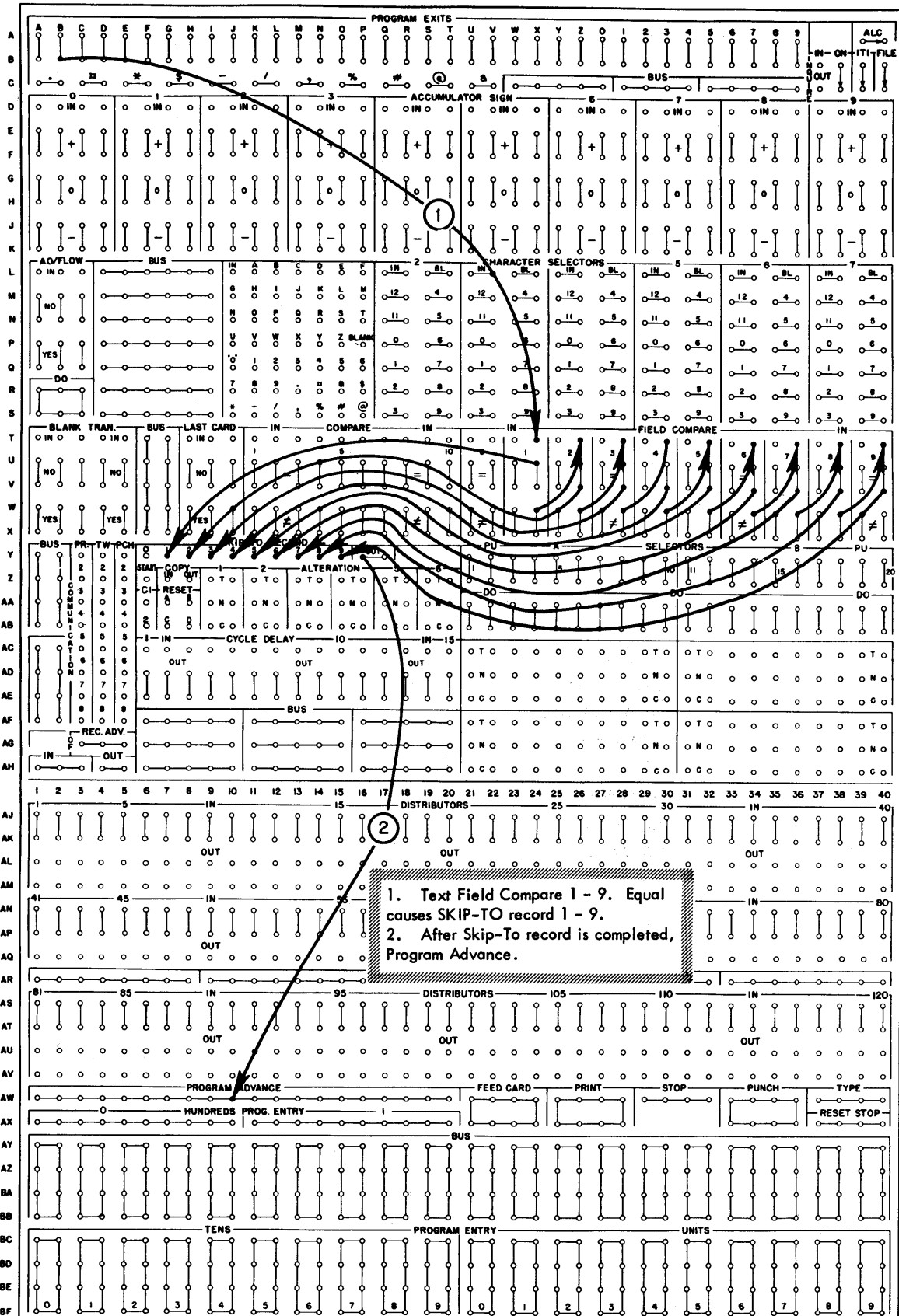
Figure 39. Wiring Diagram-Constructing an Index Record and Storing a Record (Part 2)
