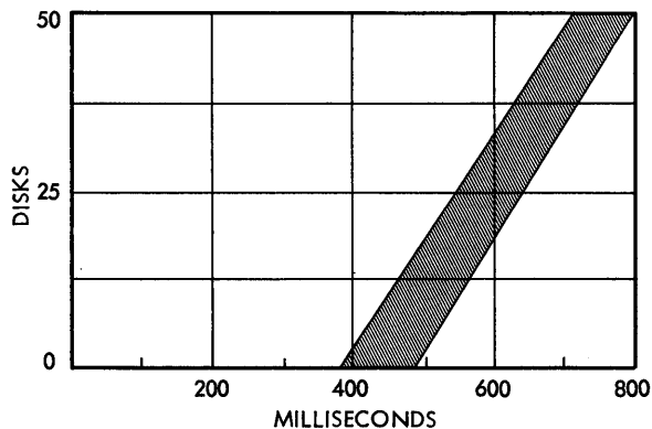
Figure 147. Seek Time for Access Arm moving from track on one disk to track on another disk
