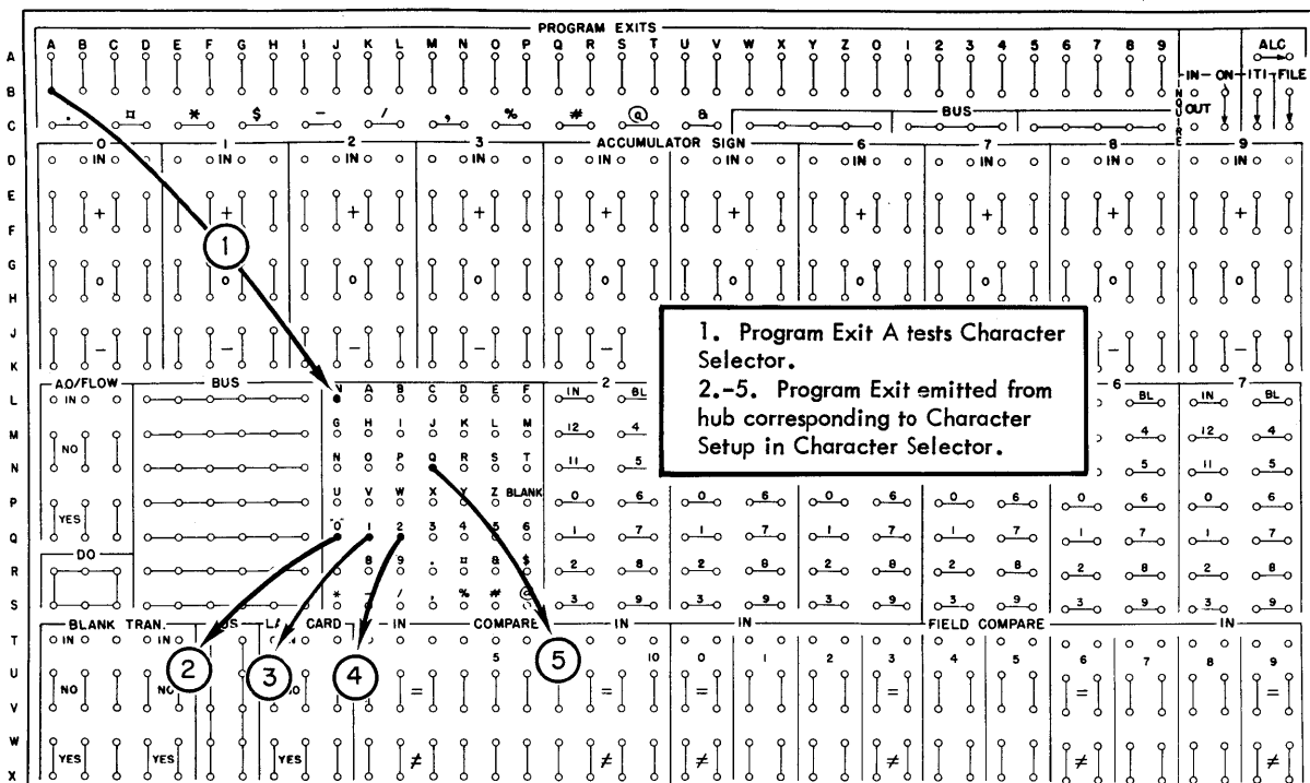
Figure 121. Program Exit Expansion-Character Selector
