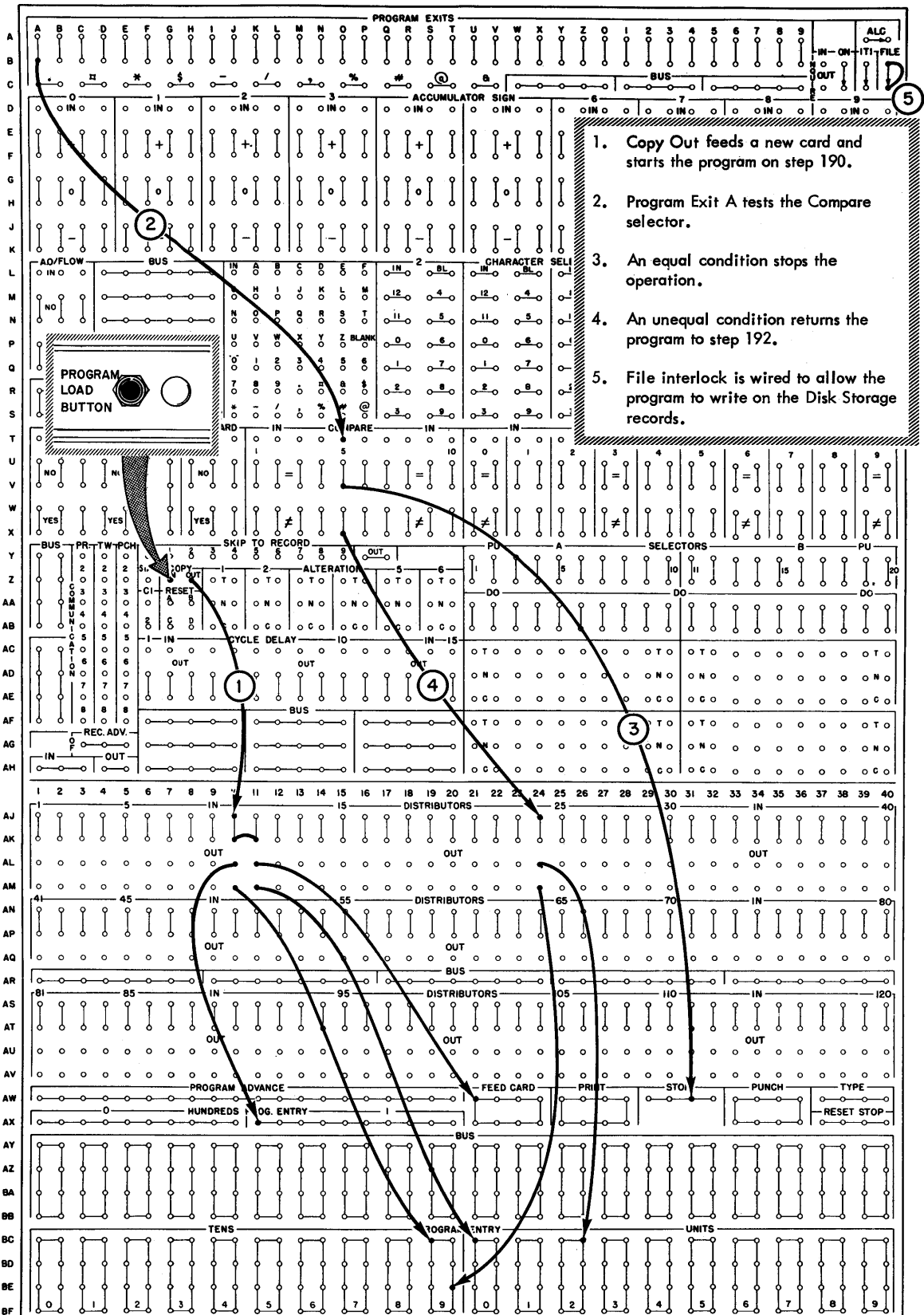
Figure 30. Control Panel Wiring for Clearing Disk Storage
