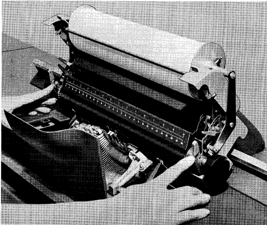
Figure 73. Removing the Platen
