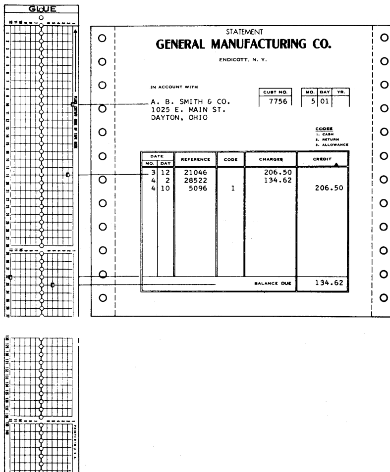
Figure 84. Control Tape
