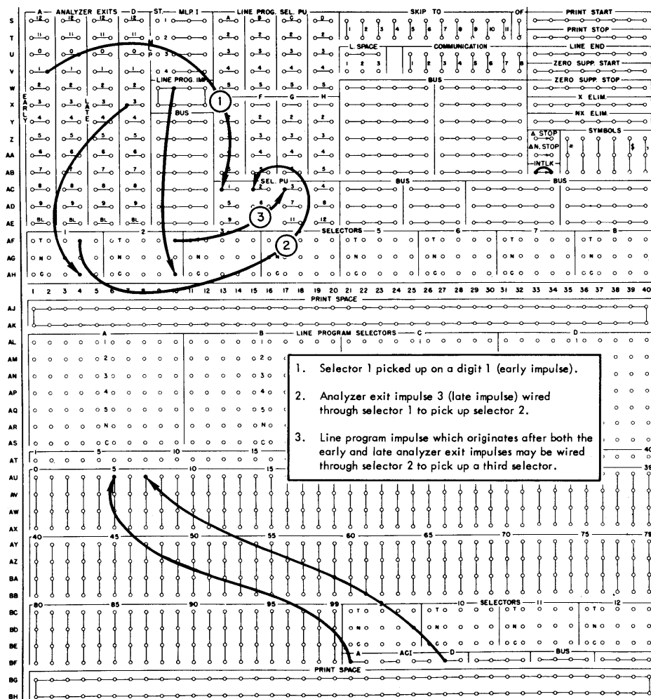
Figure 100. Series Wiring to Illustrate Timings
