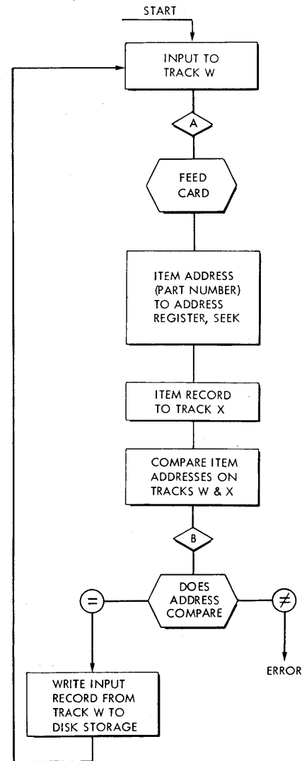
Figure 32. Block Diagram of a Disk Storage Loading Program
