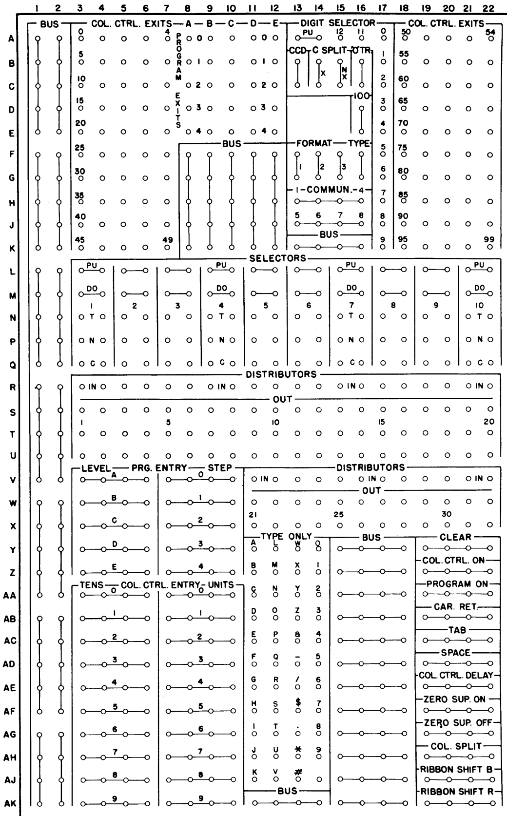
Figure 62. 380 Typewriter Control Panel
