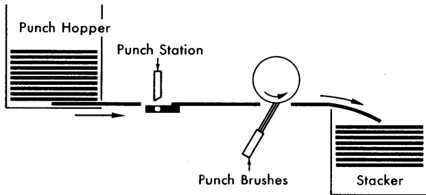
Figure 103. Punch Feed Schematic
