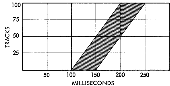
Figure 146. Seek Time for Access Arm moving from one track to another track on same disk
