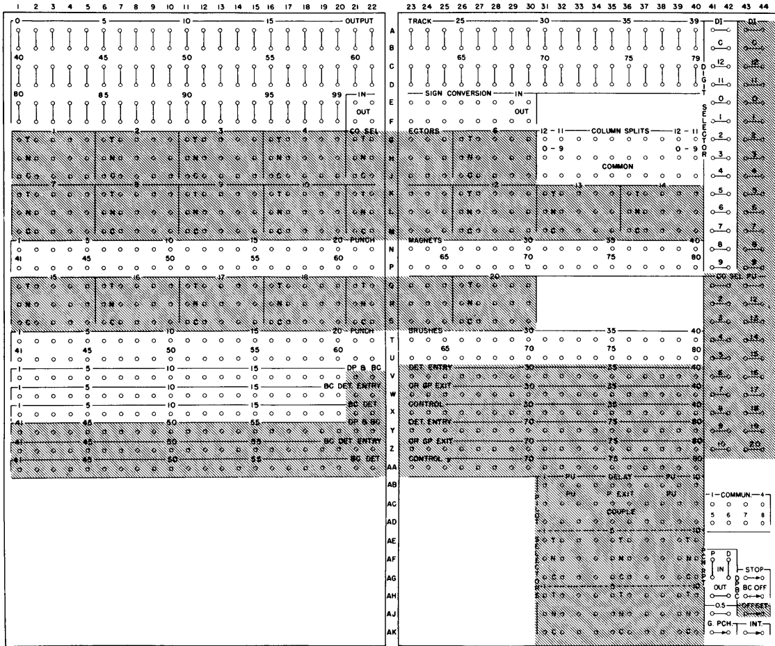
Figure 105. 323 Punch Control Panel
