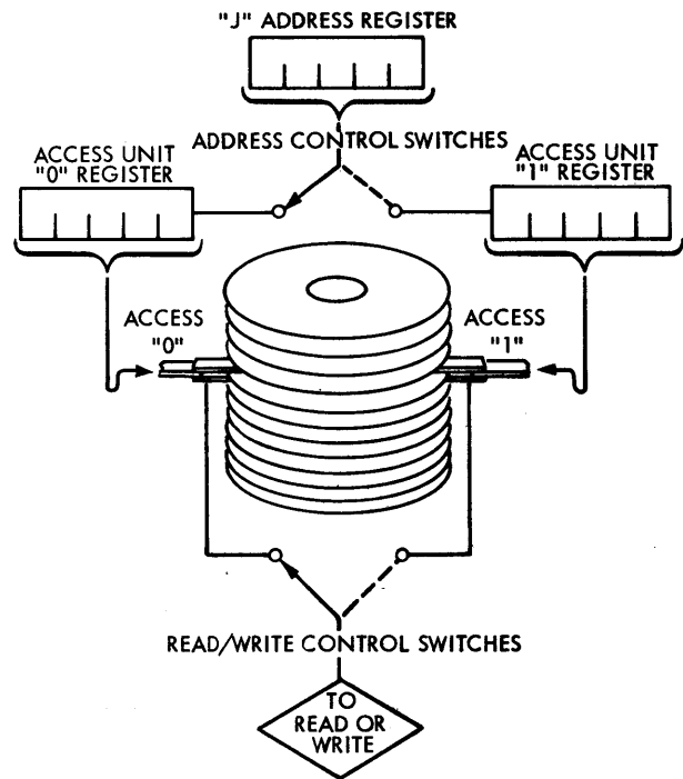
Figure 136. Schematic of Dual Access Units
