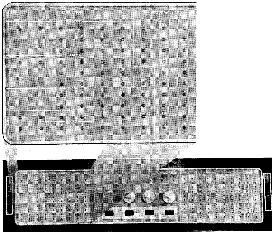
Figure 57. Program Instruction Lights
