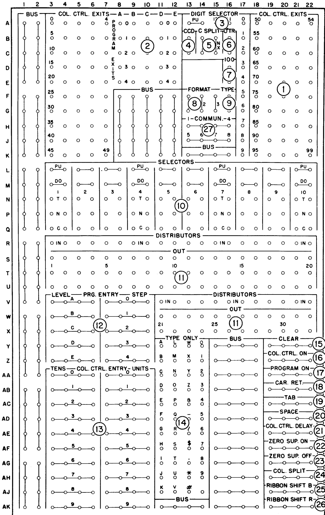
Figure 145. 380 Console Control Panel — Form 22-6329
