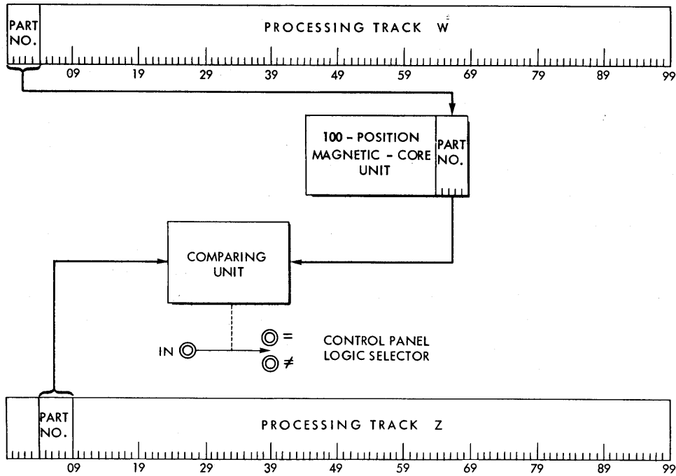
Figure 18. Schematic of a Comparing Operation
