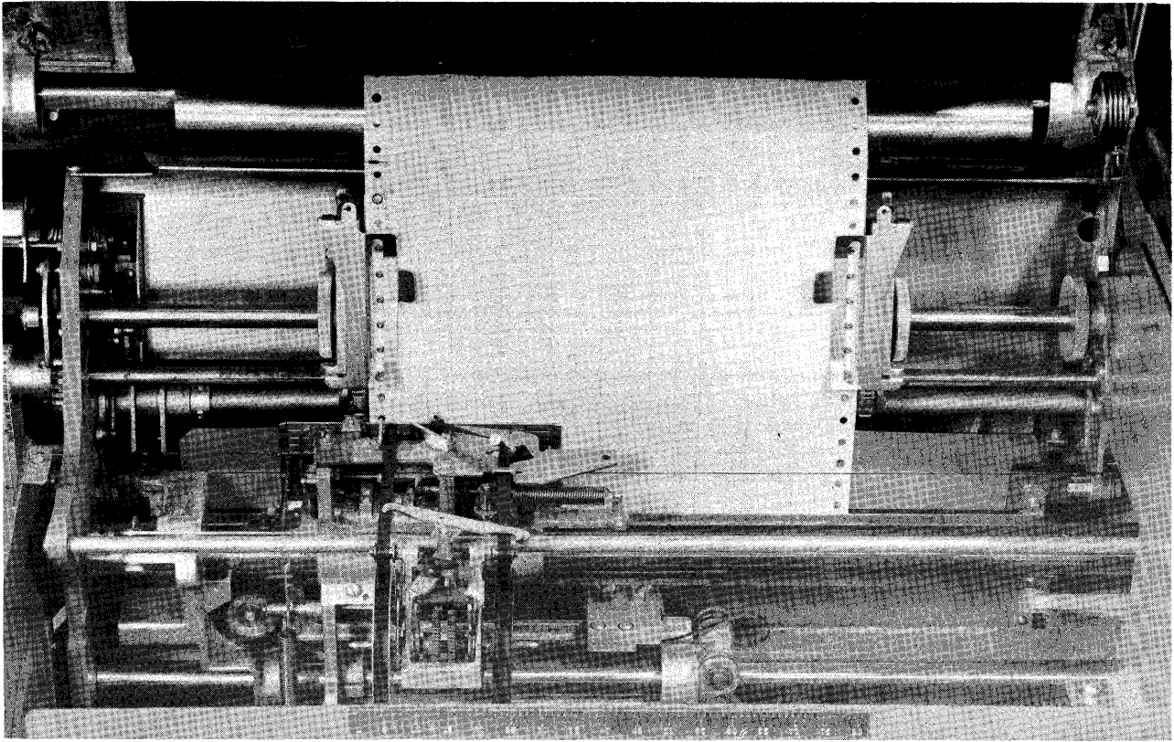
Figure 83. Tape-Controlled Carriage
