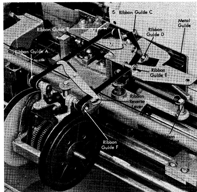
Figure 93. 370 Printer Ribbon
