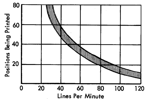
Figure 148. 370 Printer Speeds
