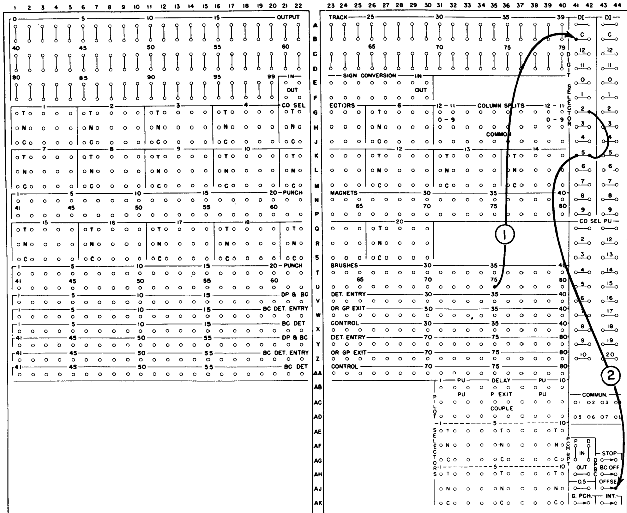
Figure 128. Off-setting Different Types of Cards
