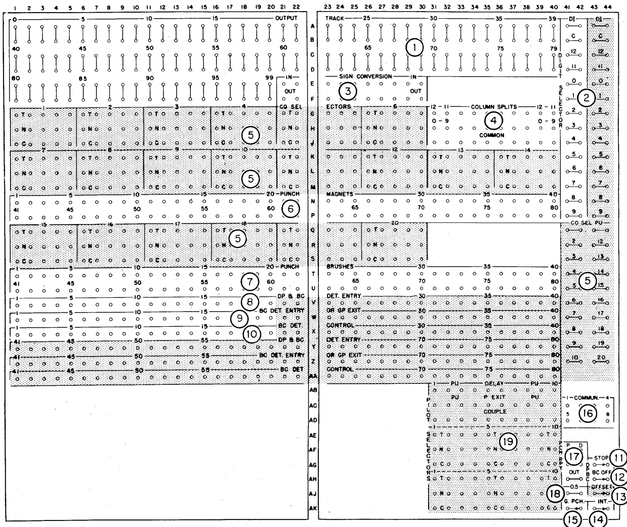
Figure 144. 323 Punch Control Panel
