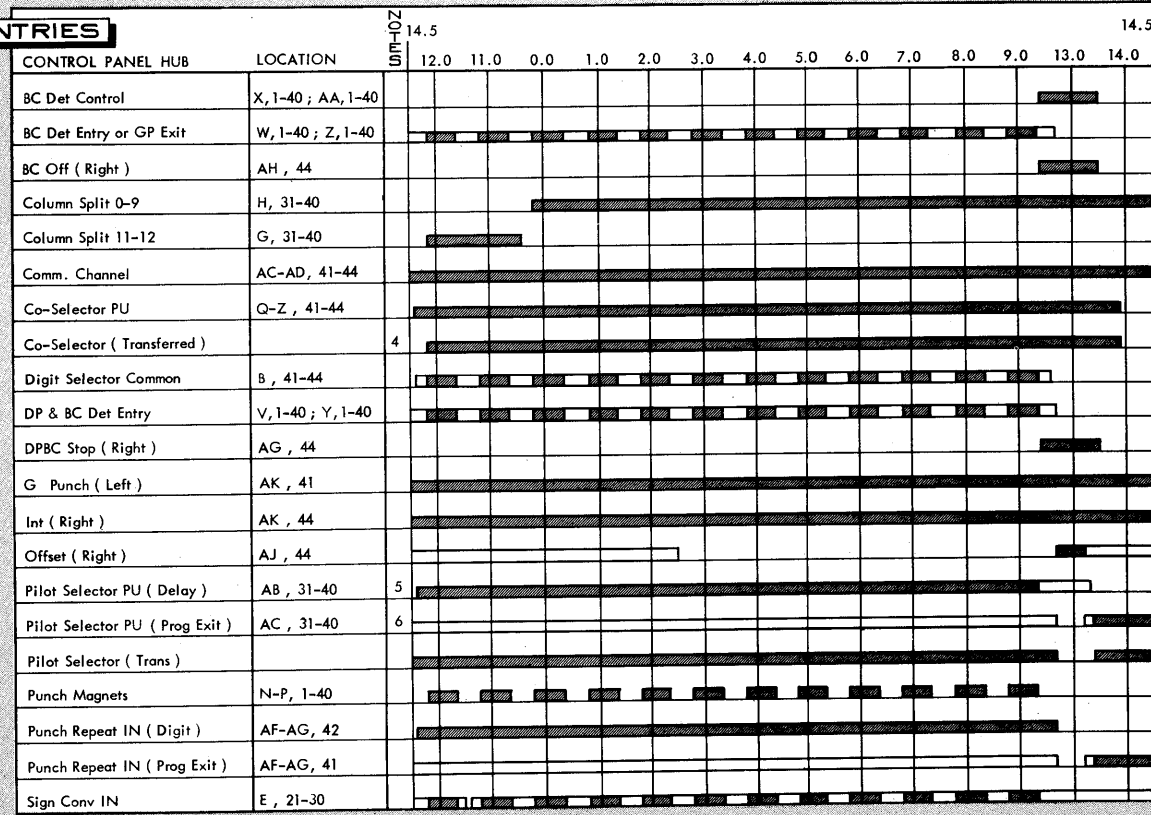
Figure 113. Timing Chart — 323 Punch
